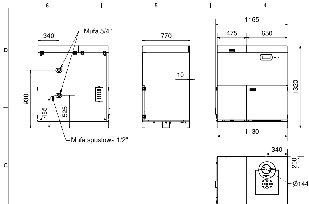
EG Pellet 10-25 kW standard - lewy
