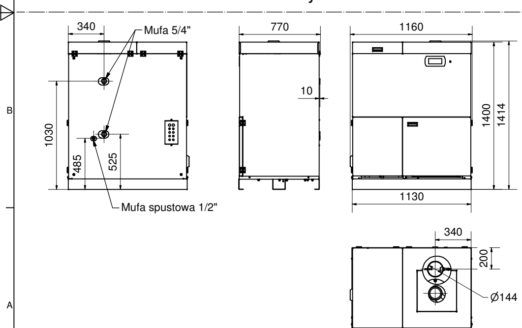
EG Pellet 10-25 kW standard - lewy
